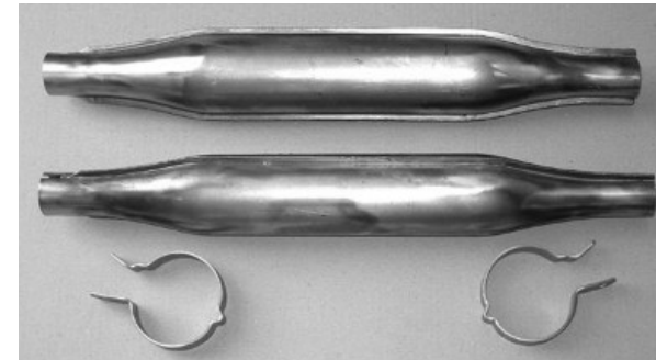
Exhaust Muffler, Trumpet-Style, Cr (like original for K-750) Fits Left and Right Side Vendor ID: S16 List Price: €75.99 ( www.ural-zentrale.de ) Long Down-Pipes Needed
