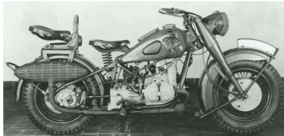
BMW R75 with Standard High-Mount Muffler
