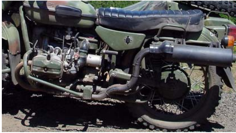
First High-Pipe (ver. 1.2), Built in Early 2006 from Muffler Off Kawasaki 750 V-Twin Quad. Muffler Was Very Heavy , But Cheap.
