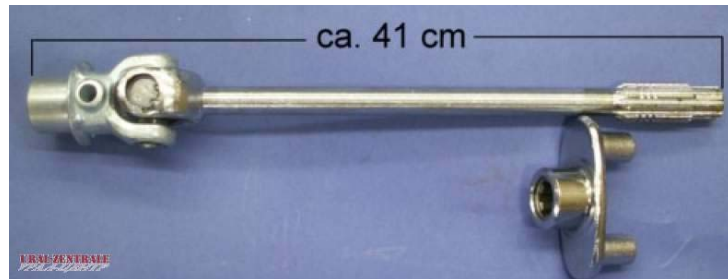
Final drive shaft (cardan shaft), Cr With joint for M-72 and some Dnepr and Ural models Overall length: 41cm Final drive shaft, chrome-plated Vendor ID: S872-KUE List Price: €59.89 ( www.ural-zentrale.de )
