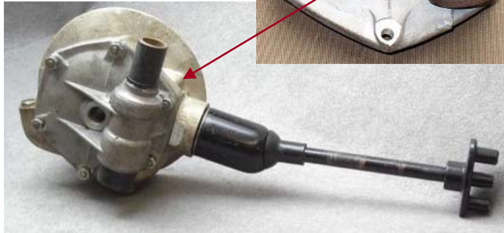
Rear Drive with Cardan Shaft, 8 X 37 Gear Ratio (M-72, German R71) Vendor #: 002.749 List Price: €315.00 ( www.oldtimergarage.eu )
