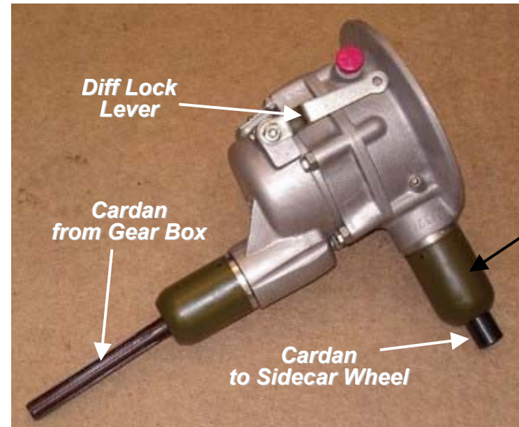
Rear Drive with Locking Differential (MB-750, MT-12) Vendor ID: 002.125 List Price: €1,050.00 (www.oldtimergarage.eu)
