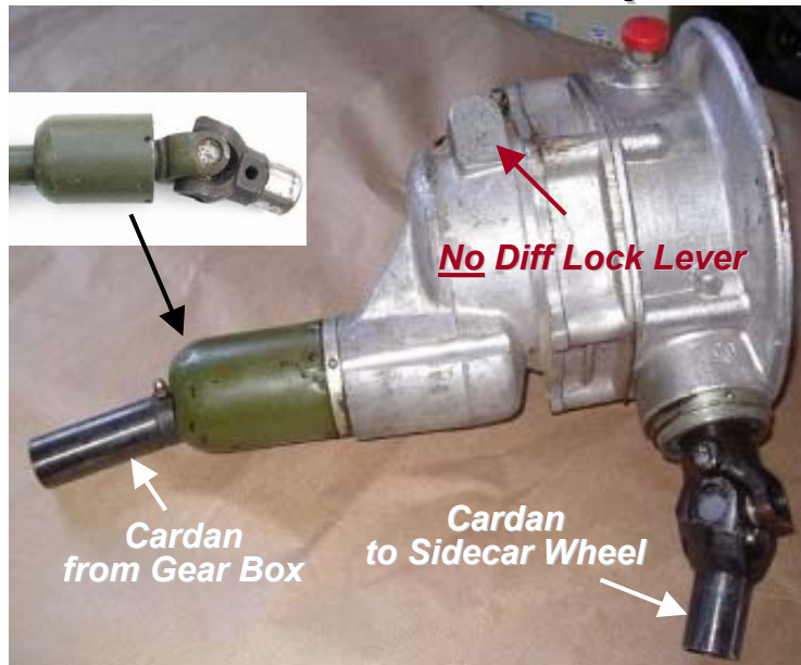
Rear Drive Vendor #: 002.122 (MB-750, MB-650, MT-16, MT-12) List Price: €850.00 (www.oldtimergarage.eu)
