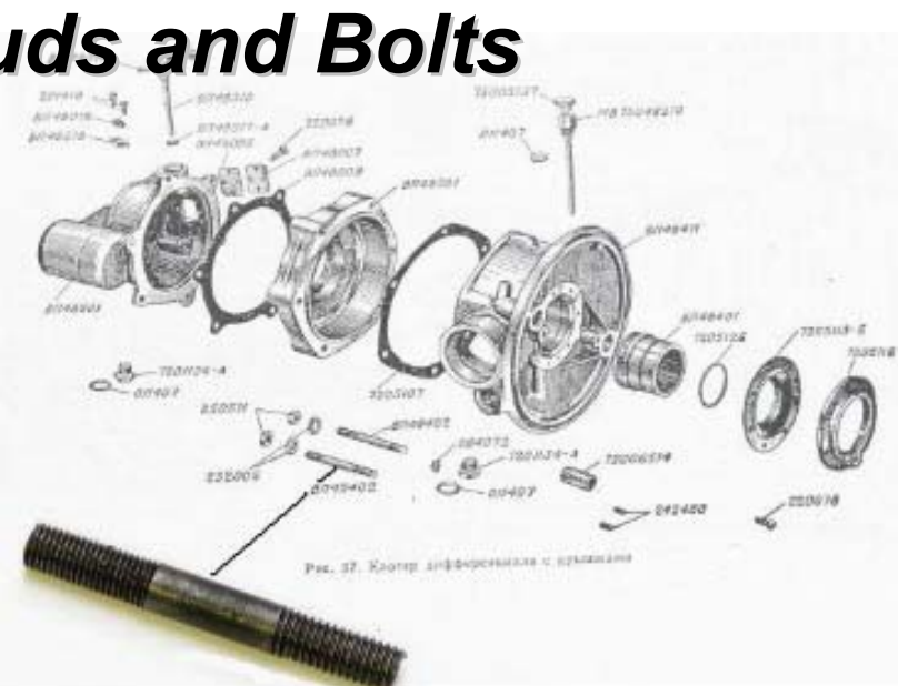
Rear Drive Stud M8 x 60 (MB-750) Part ID: BП48402 Vendor #: 000.653 List Price: €2.02 (www.oldtimergarage.eu)
