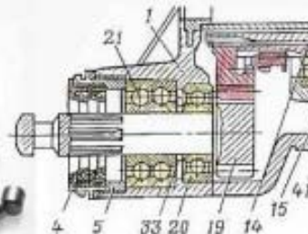
Rear Drive Bearings Set #2 (Old Type) (MB-750, MB-650) Vendor #: 003.213 List Price: €95.00 ( www.oldtimergarage.eu )
